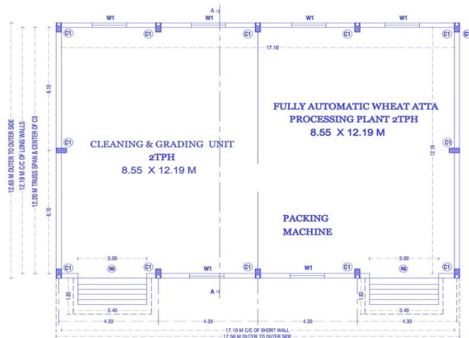
FACTORY SHED PLAN
